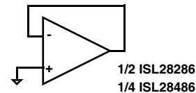
FIGURE 37. PREVENTING OSCILLATIONS IN UNUSED CHANNELS
